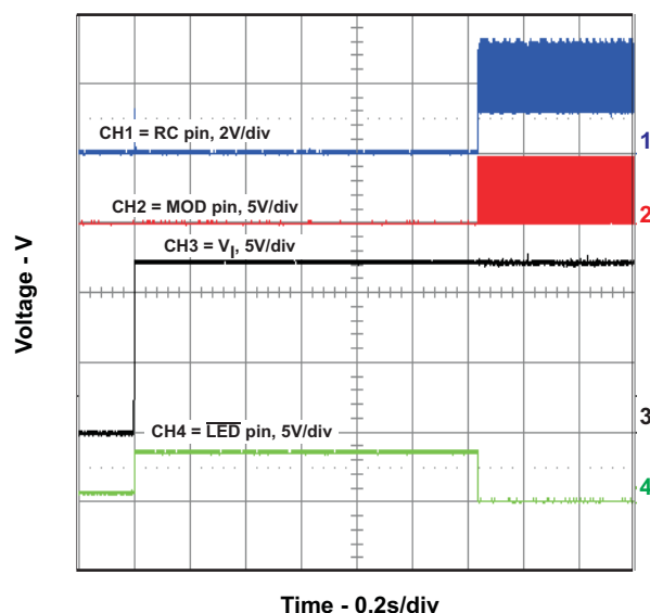
Figure 13. bq2000 Start-up on Vin
