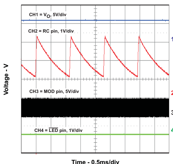
Figure 15. bq2000 in Fast Charge
