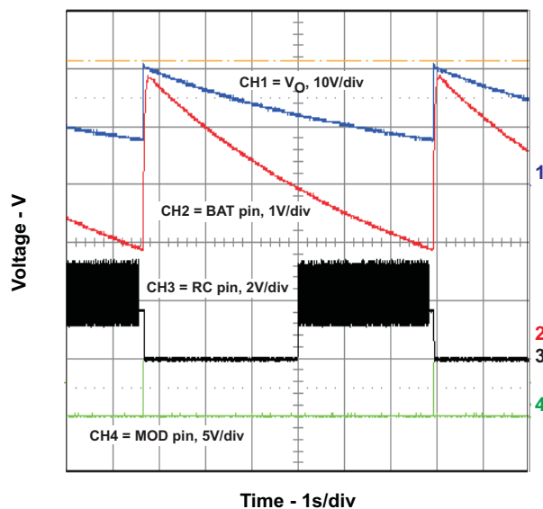
Figure 18. bq2000 in Sleep Mode
