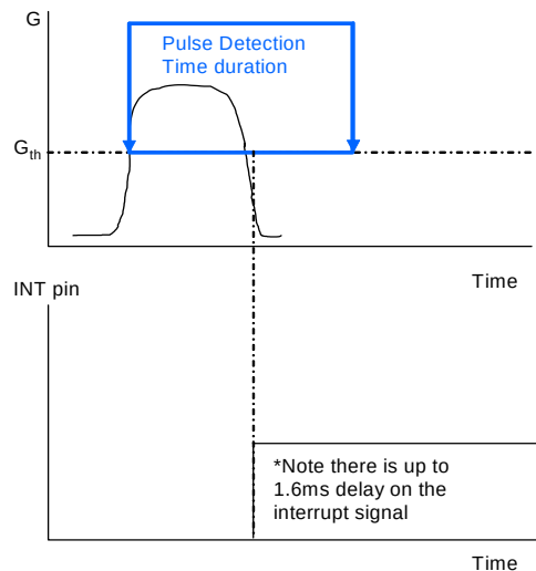
Figure 3. Single Pulse Detection
