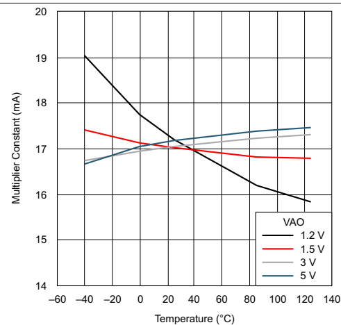
Figure 6. Multiplier Constant vs Junction Temperature
