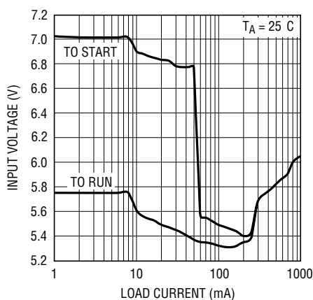
(7a) Typical Minimum Input Voltage, V_{\text{OUT}} = 5\text{V} , f_{\text{SW}} = 750\text{kHz}
