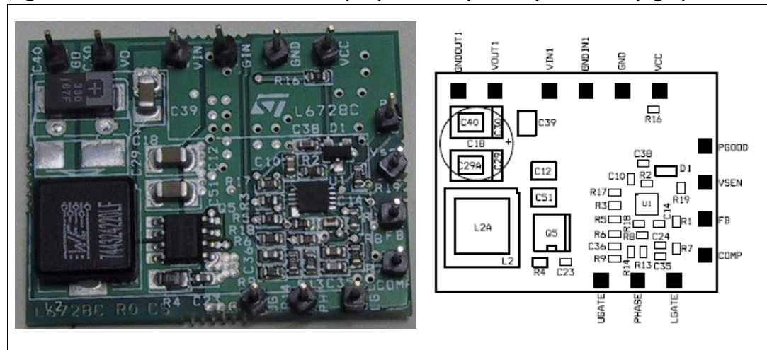
Figure 15. 5 A demonstration board (left) and component placement (right)
