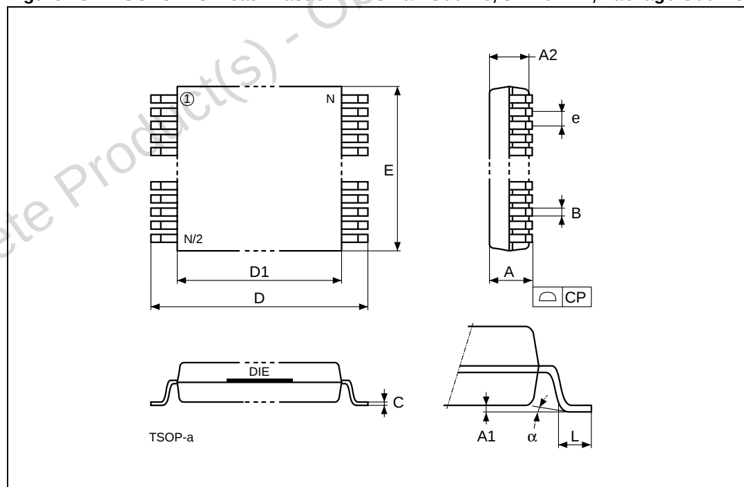
Figure 13. TSOP32 - 32 lead Plastic Thin Small Outline, 8 x 20 mm, Package Outline
