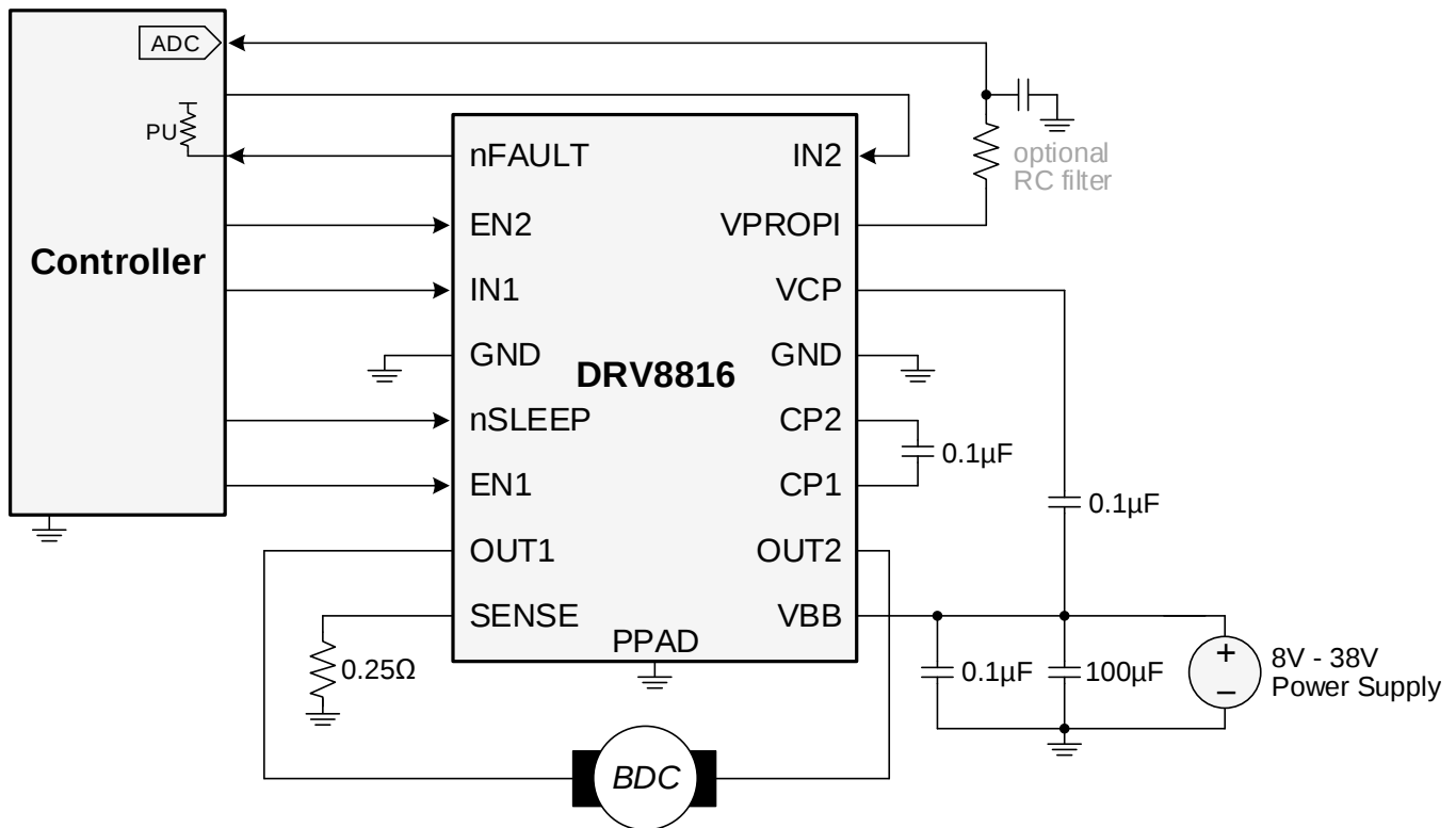
Figure 7. Typical Application
