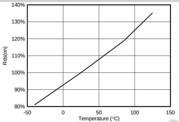
Figure 2. R DS(ON) vs Temperature
