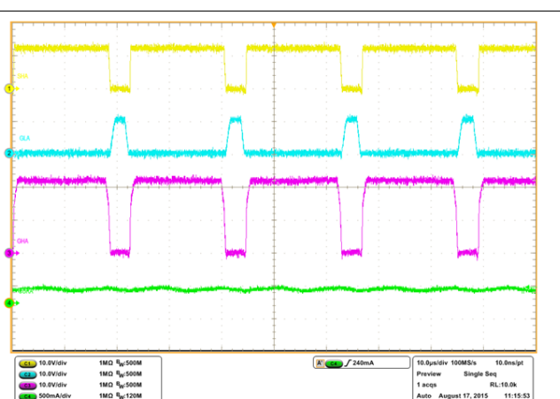
Figure 20. Gate Drive 80% Duty Cycle
