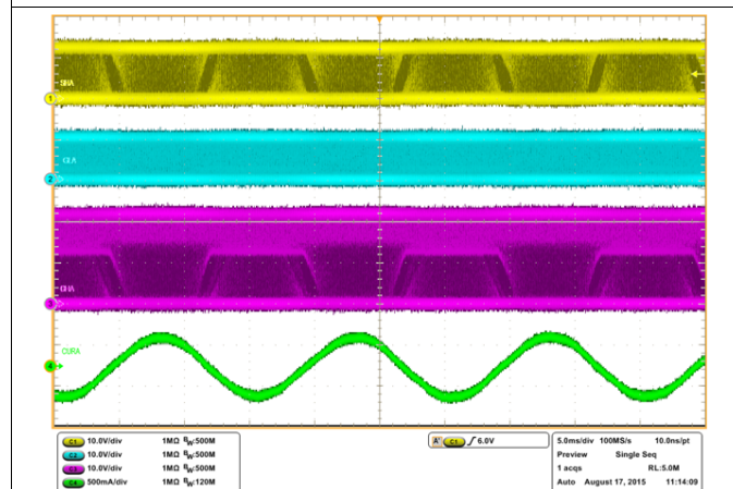
Figure 19. Gate Drive 20% Duty Cycle
