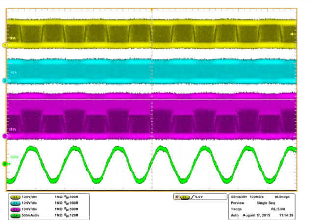
Figure 20. Gate Drive 80% Duty Cycle
