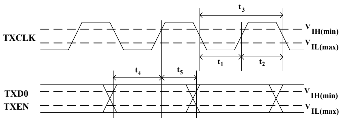
Figure 10. SNI Transmission Cycle Timing-1
