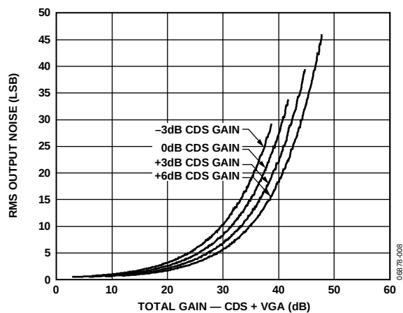
Figure 8. Output Noise vs. Total Gain (CDS + VGA)
