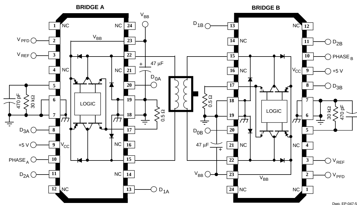
Figure 4 — Typical Application
