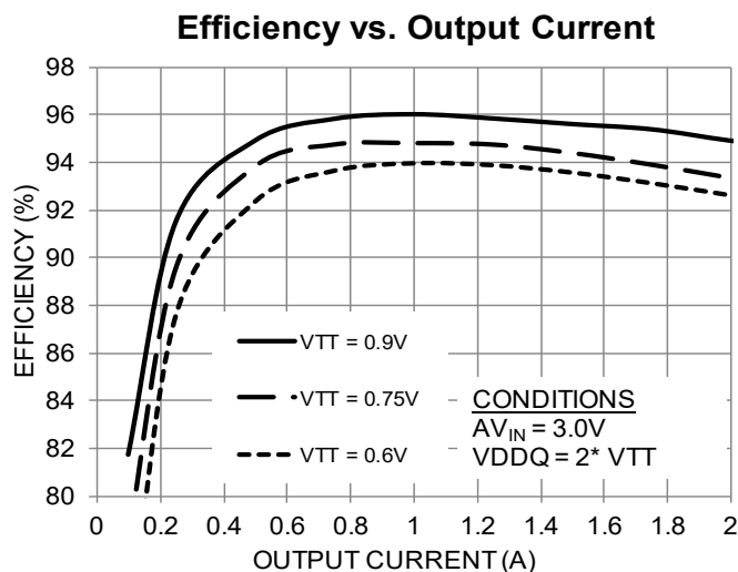
Figure 2: Highest Efficiency in Smallest Solution Size
