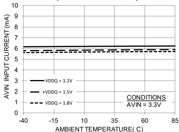
AVIN Input Current vs. Temperature
