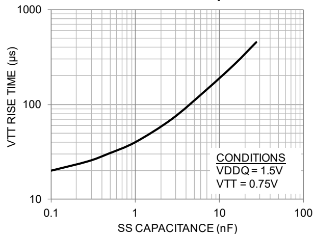
VTT Rise Time vs. Capacitance
