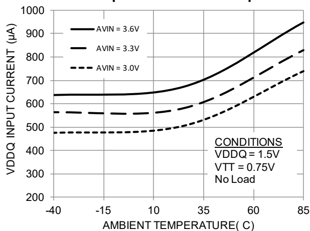
VDDQ Input Current vs. Temperature
