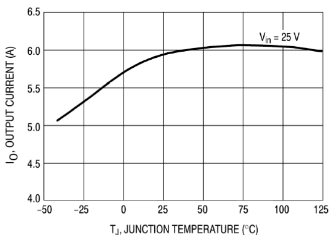
Figure 5. Current Limit
