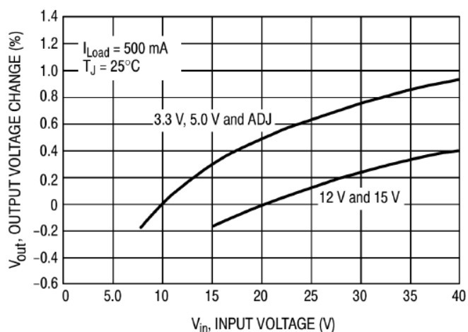
Figure 3. Line Regulation
