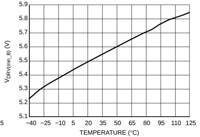
Figure 13. Minimal Driver High Level – B Version, V_{CC} = V_{CC\_OFF} + 0.2\text{ V} and C_{load} = 0\text{ nF}
