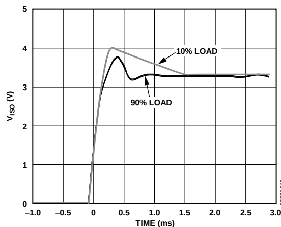
Figure 13. Typical Output Voltage Start-Up Transient at 10% and 90% Load, V_{ISO} = 3.3V
