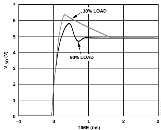
Figure 12. Typical Output Voltage Start-Up Transient at 10% and 90% Load, V_{ISO} = 5V
