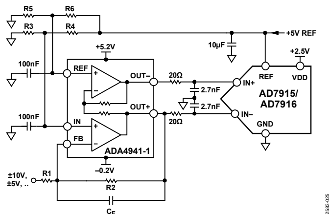
Figure 33. Single-Ended to Differential Driver Circuit
