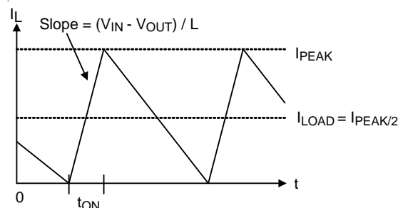
Figure 6. Boundary condition of CCM/DEM
