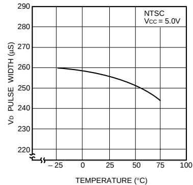
Fig. 16 V b pulse width vs. temperature
