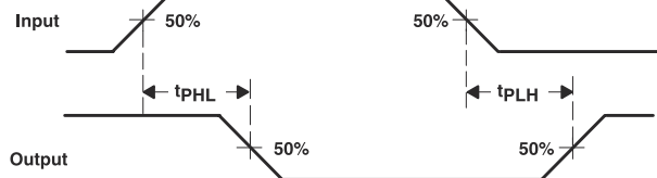
VOLTAGE WAVEFORMS
