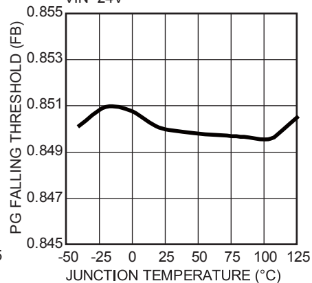
PG Falling Threshold vs. Junction Temperature VIN=24V
