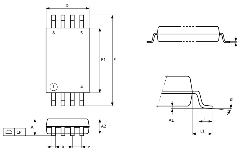
Figure 80. TSSOP8 – Outline
