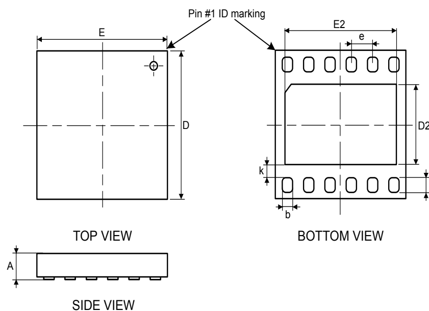
Figure 83. UFDFPN12 - Outline
