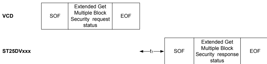
Figure 54. Extended Get Multiple Block Security Status frame exchange between VCD and ST25DVxxx
