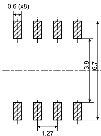
Figure 79. SO8N - Recommended footprint
