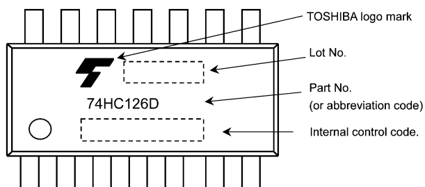
74HC126D
