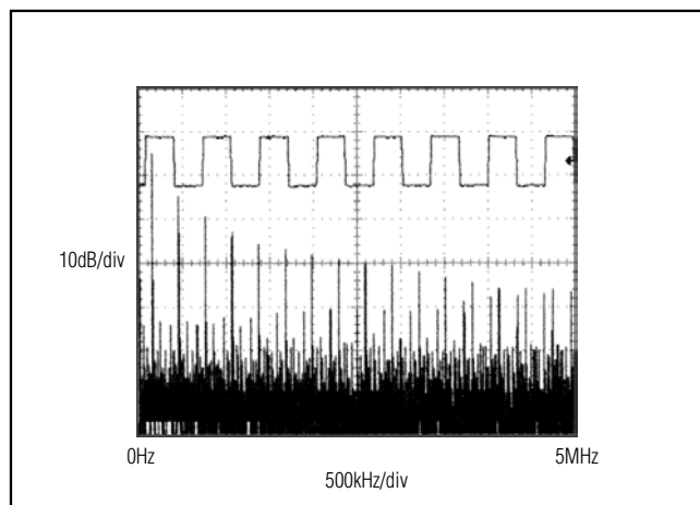
Figure 12. Driver Output Waveform and FFT Plot of MAX481/MAX483/MAX485/MAX487-MAX489 Transmitting a 150kHz Signal
