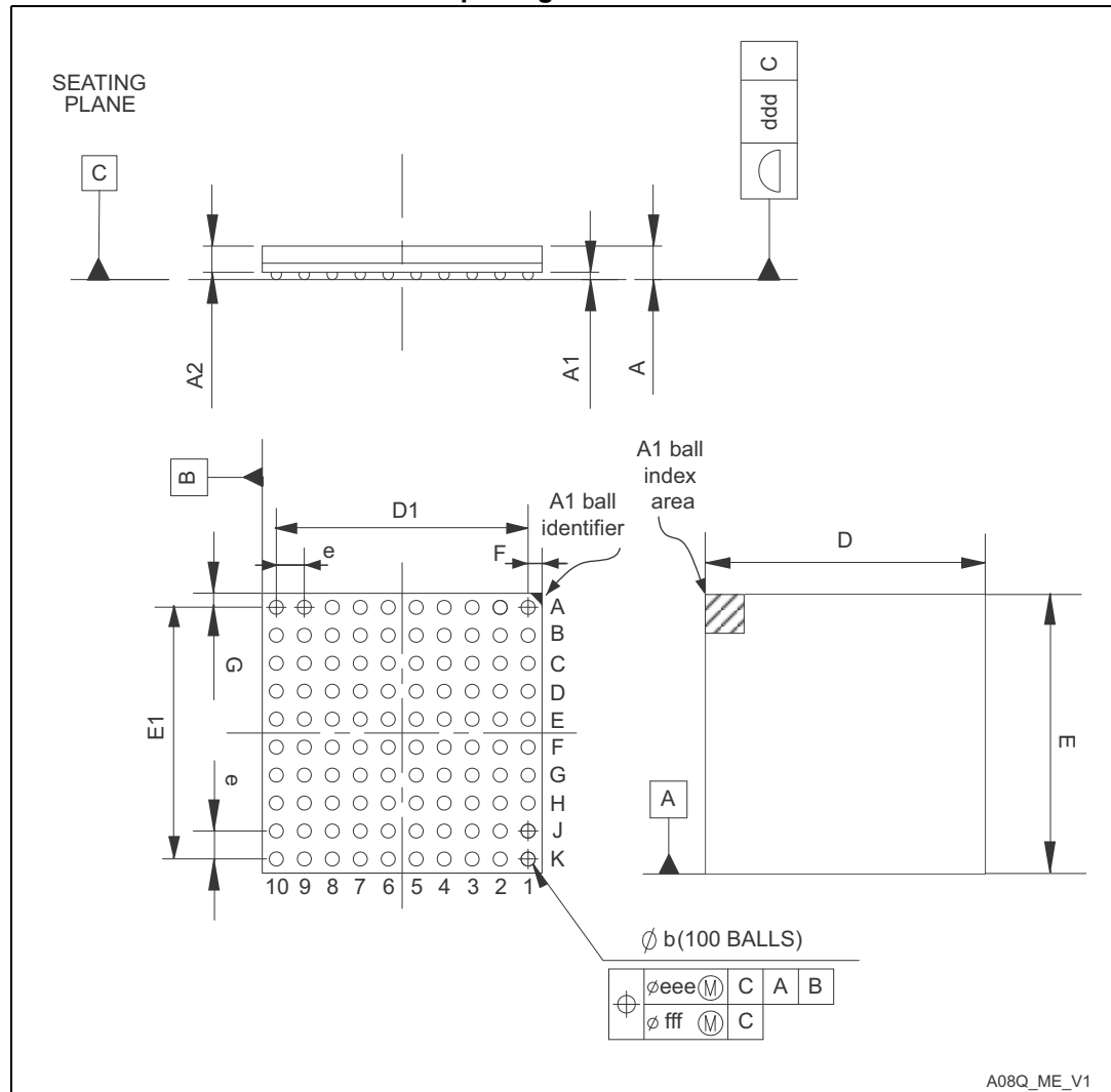
Figure 82. TFBGA100, 8 × 8 × 0.8 mm thin fine-pitch ball grid array package outline
